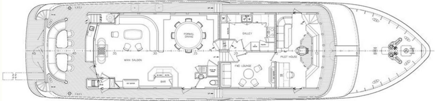
MAIN DECK
