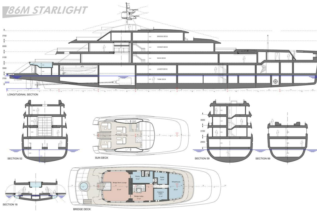
Profile, Sun and Bridge decks
