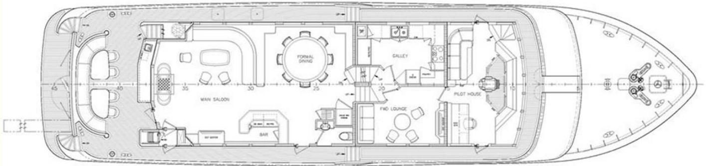
MAIN DECK
